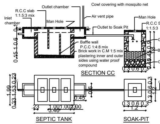
SEPTIC TANK
