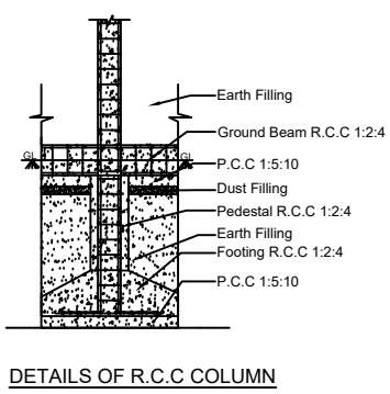
DETAILS OF R.C.C COLUMN
