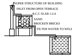
Rainwater harvesting
