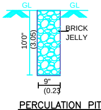
PERCOLATION PIT
