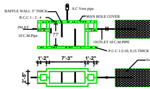
Septic tank and trench
