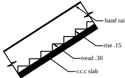
STAIR
