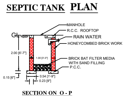
SECTION ON O - P
