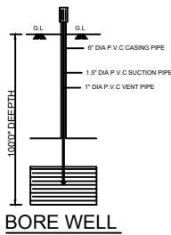
BORE WELL
