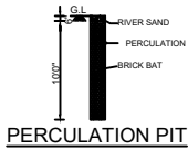
PERCOLATION PIT
