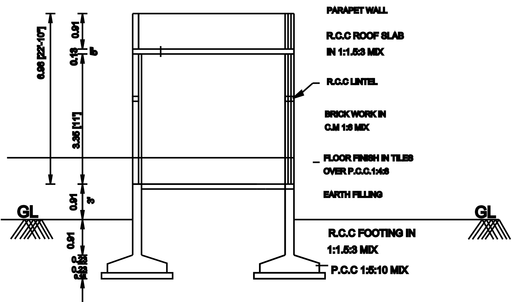
SECTION AA
