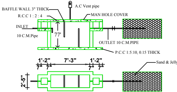
Septic tank and trench
