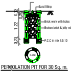
PERCOLATION PIT FOR 30 Sq. m.
