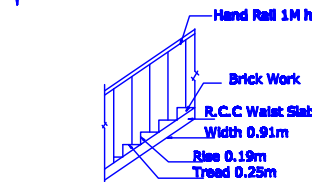
STAIRCASE DETAIL
