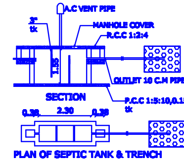
PLAN OF SEPTIC TANK & TRENCH
