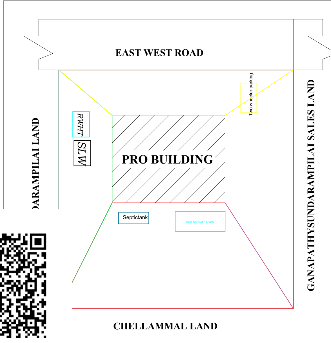
SITE PLAN
