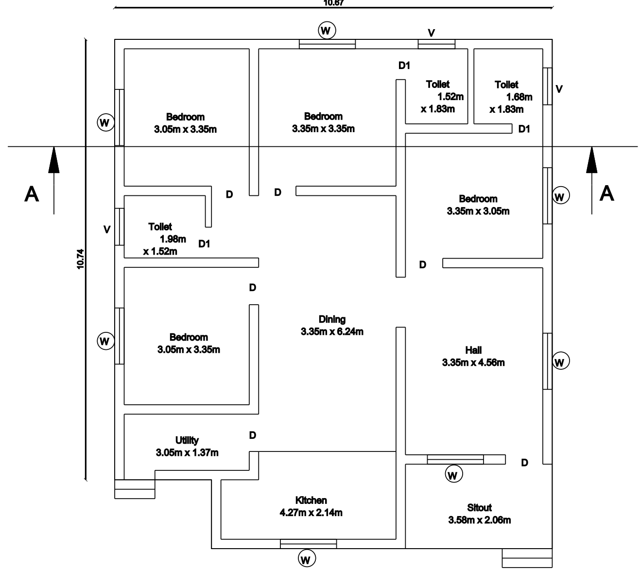
GROUND FLOOR PLAN-1
