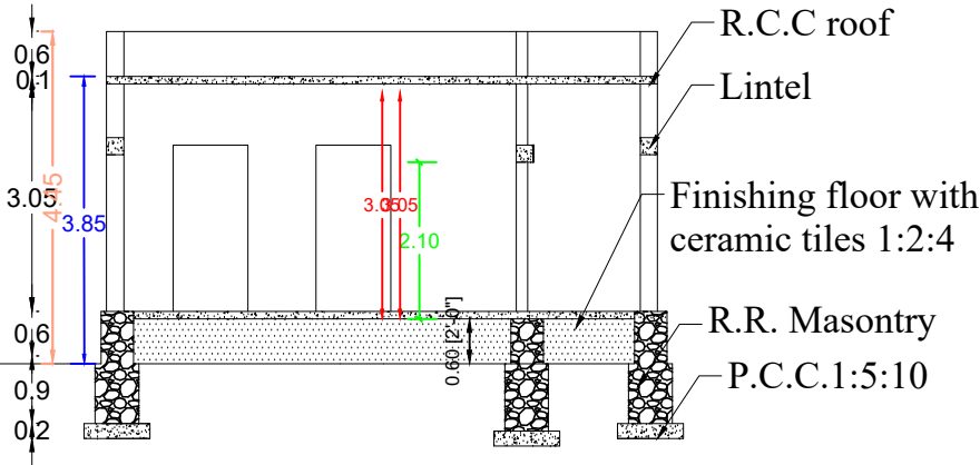
SECTION AB
