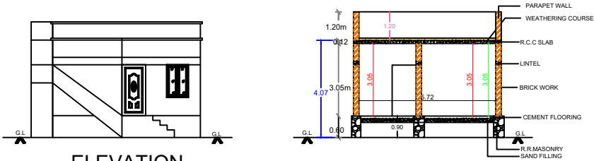
SECTION ON A-A
