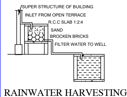
RAINWATER HARVESTING
