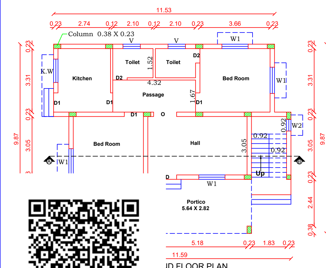
ID FLOOR PLAN
