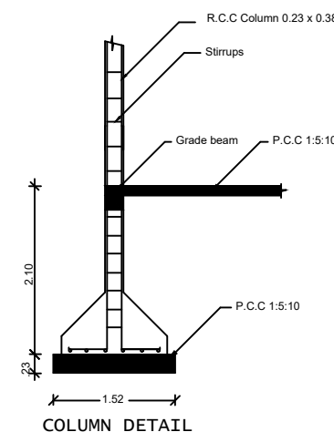
COLUMN DETAIL
