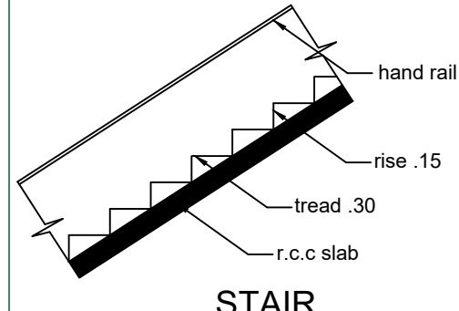
STAIR
