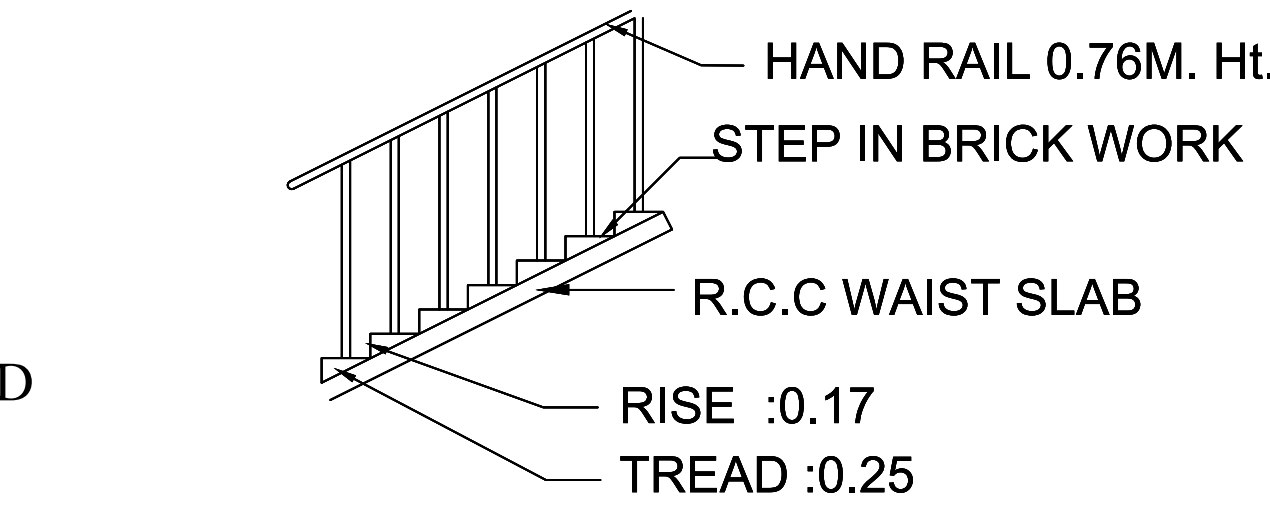
STAIR CASE DETAIL
