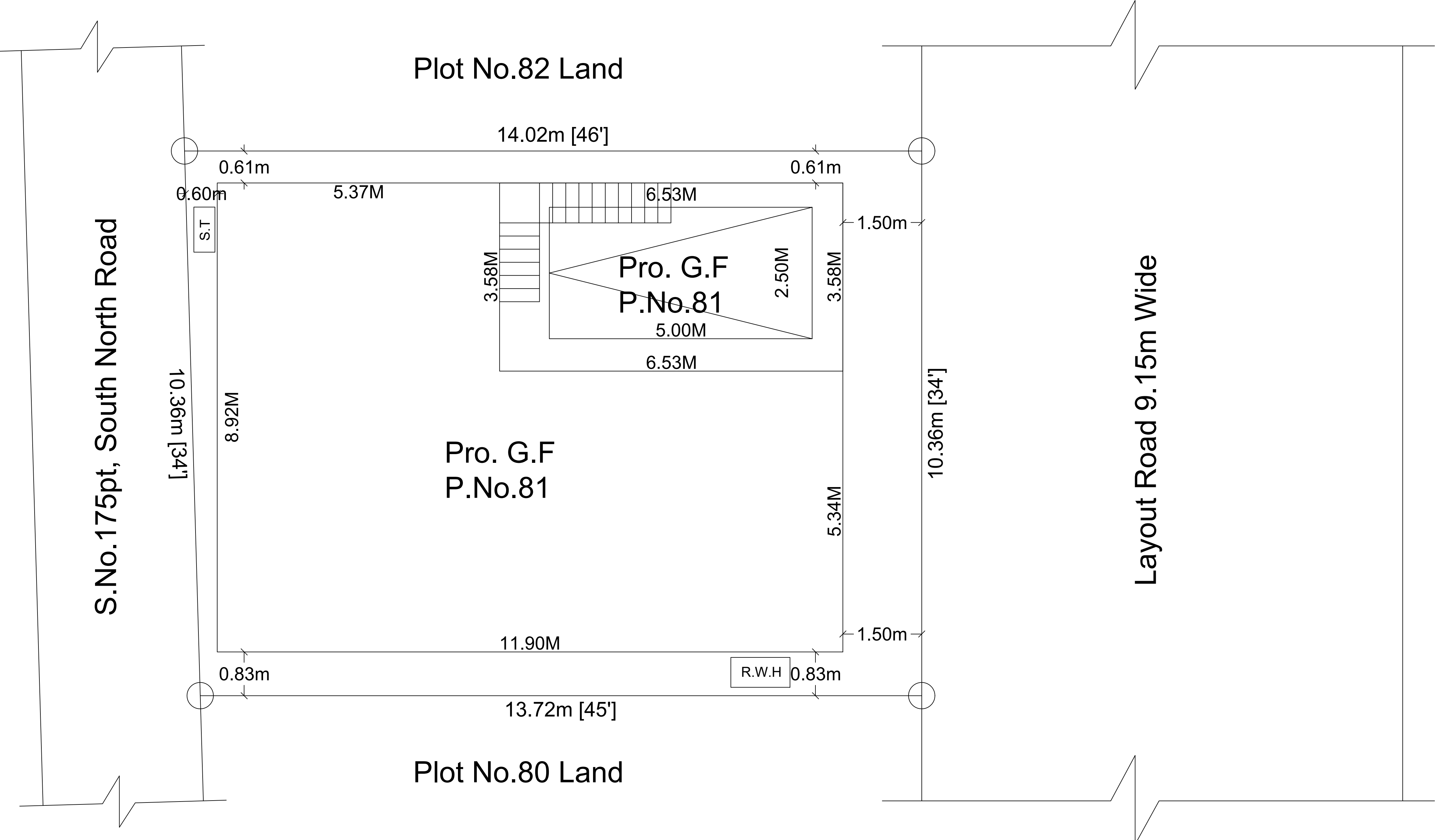
SITE PLAN
