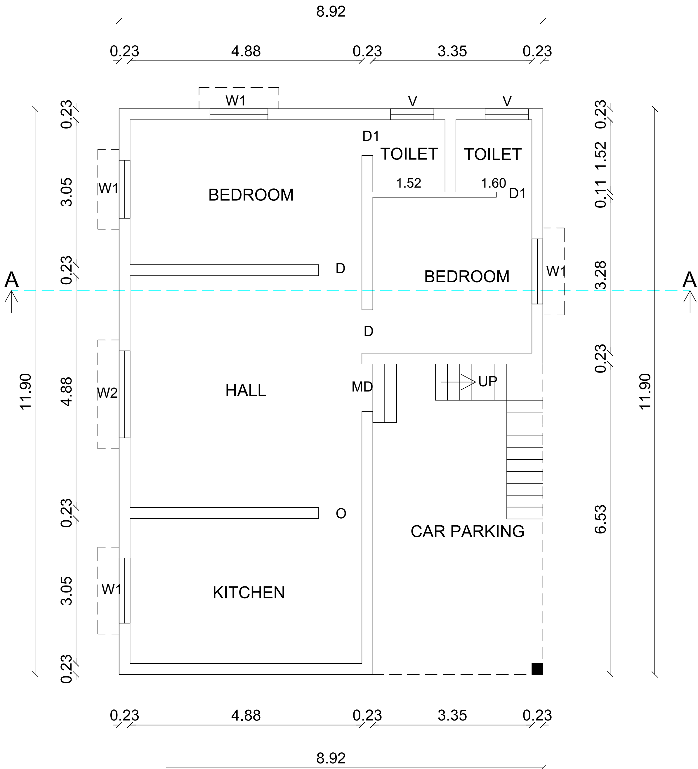
PLAN
