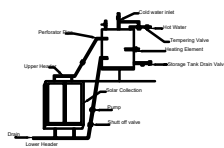
Details of solar water heater (NTS)
