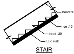
STAIR
