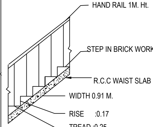
STAIR DETAIL
