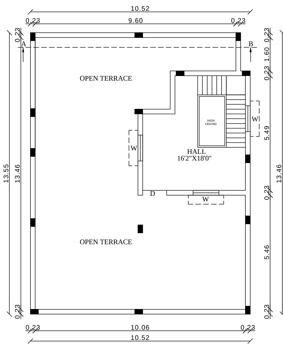
HEAD ROOM PLAN
