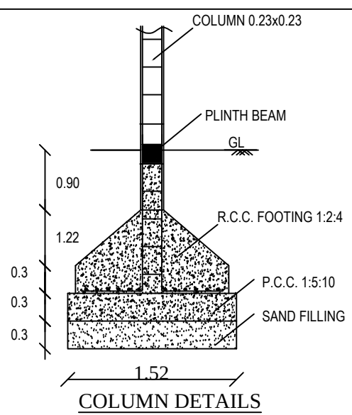
COLUMN DETAILS
