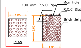
SECTION OF RAINWATER COLLECTION TANK
