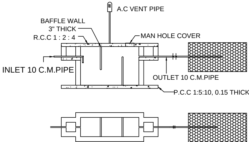
SEPTIC TANK &TRENCH
