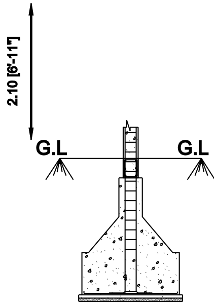
COLUMN DETAILS
