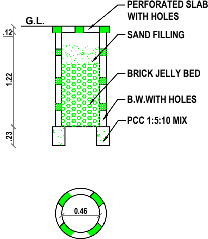
RAIN WATER HARVEST
