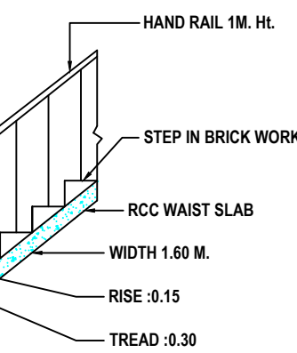
STAIR DETAIL
