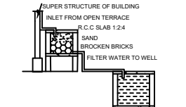
RAINWATER HARVESTING
