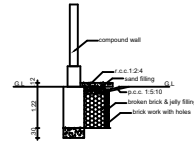
PLINTH BOUNDARY PERCOLATION PIT
