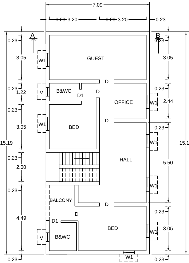
FF PLAN
