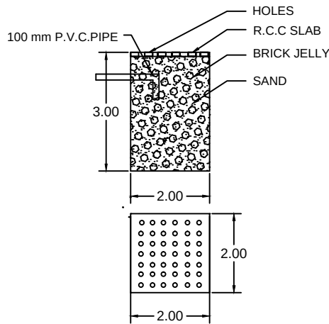
RAIN WATER COLLECTING TANK
