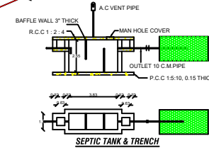
SEPTIC TANK & TRENCH
