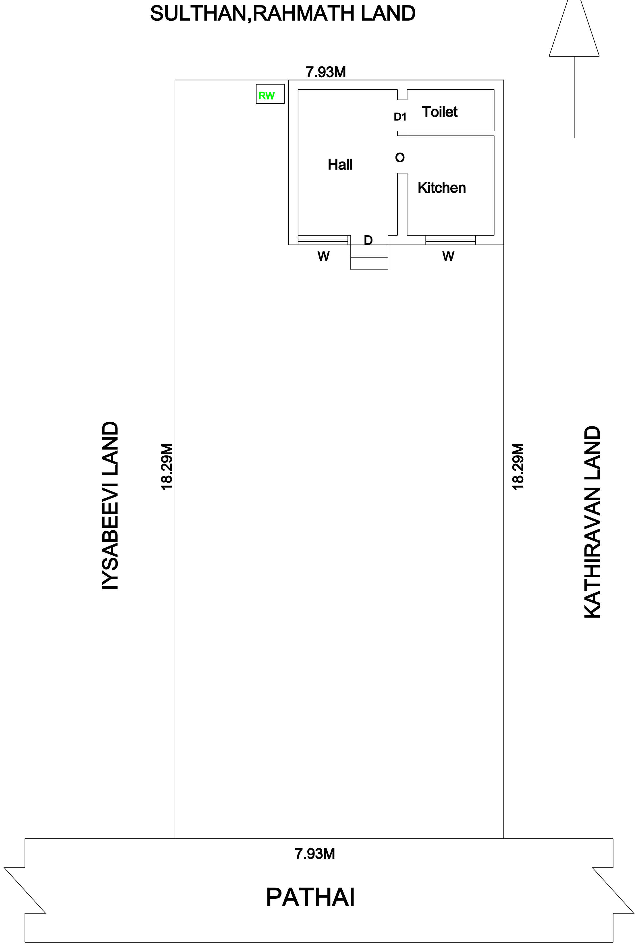
SITE PLAN
