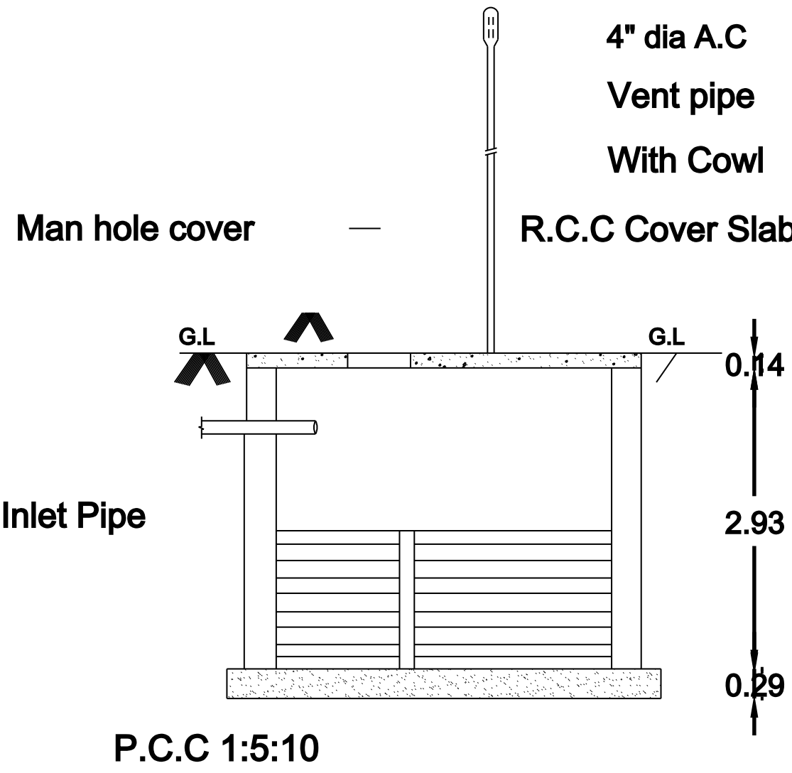
SECTION
