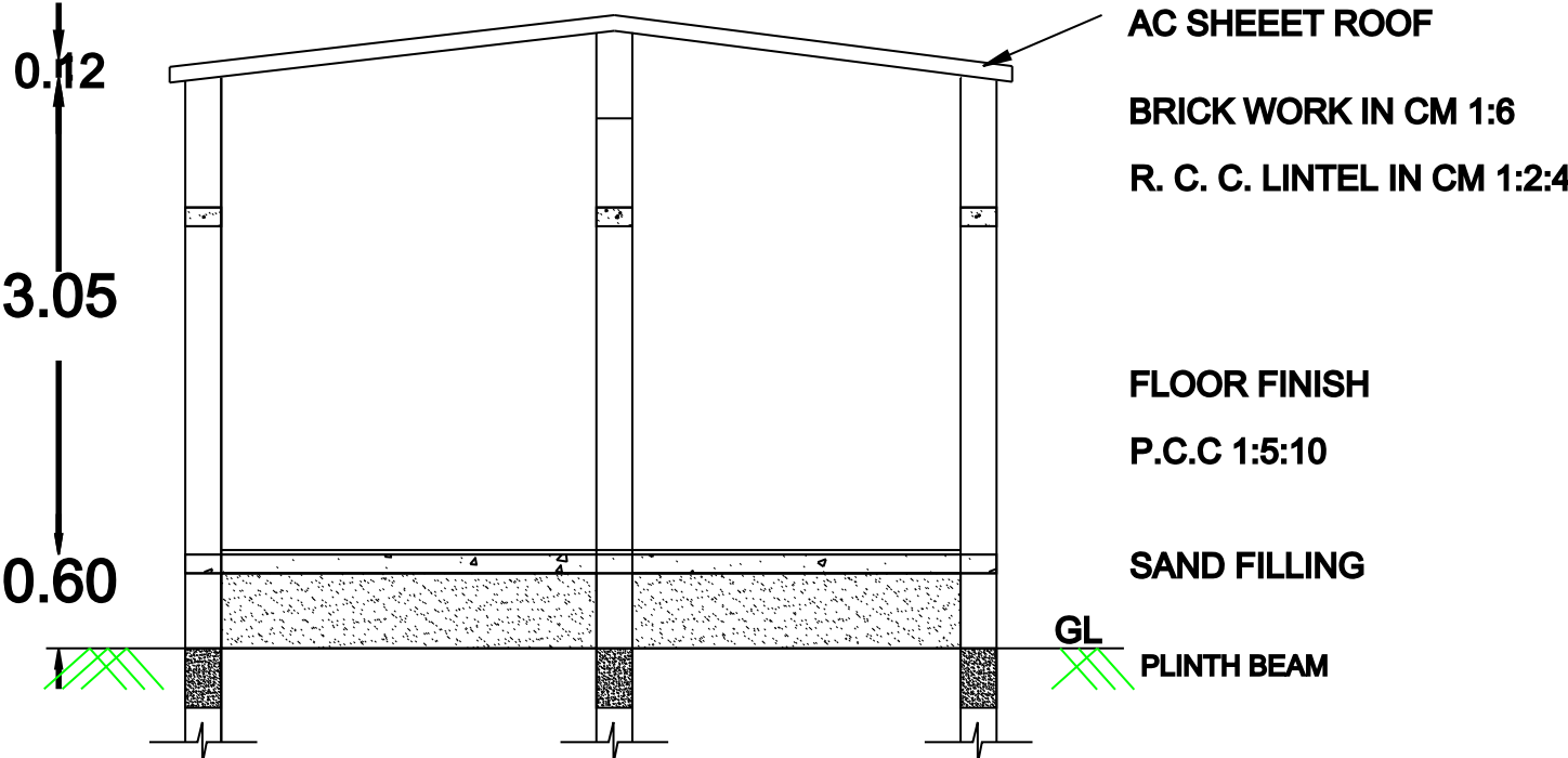
SECTION
