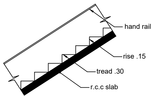
STAIR
