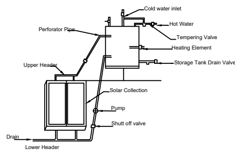
Details of solar water heater (NTS)
