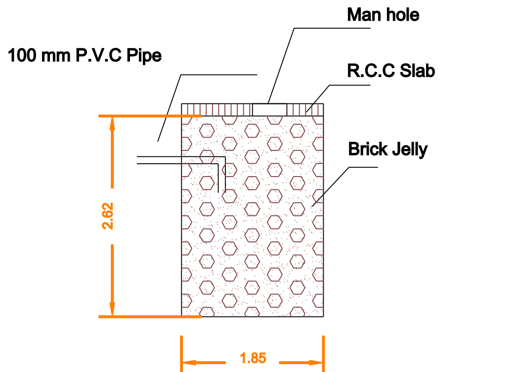
SECTION OF RAINWATER COLLECTION TANK
