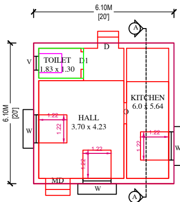
PRO.GOUND FLOOR PLAN
