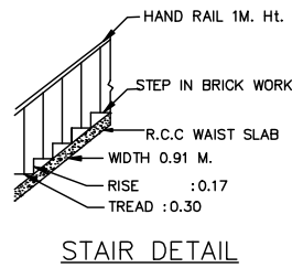
STAIR DETAIL
