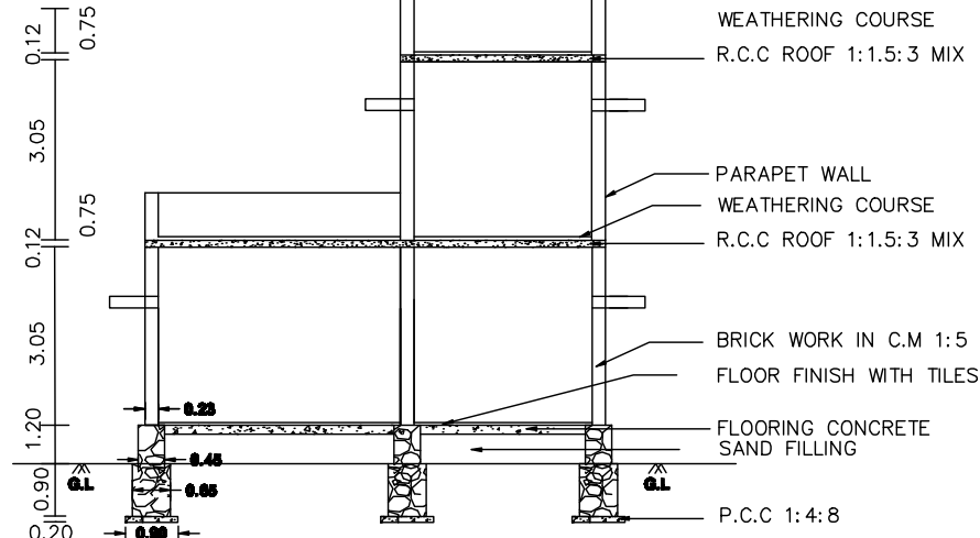
SECTION AB
