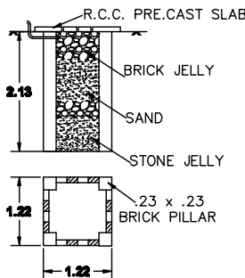
PLAN & SECTION OF RAIN WATER COLLECTION WELL
