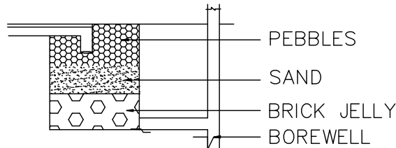
RAINWATER FILTRATION
