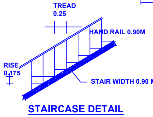
STAIRCASE DETAIL
