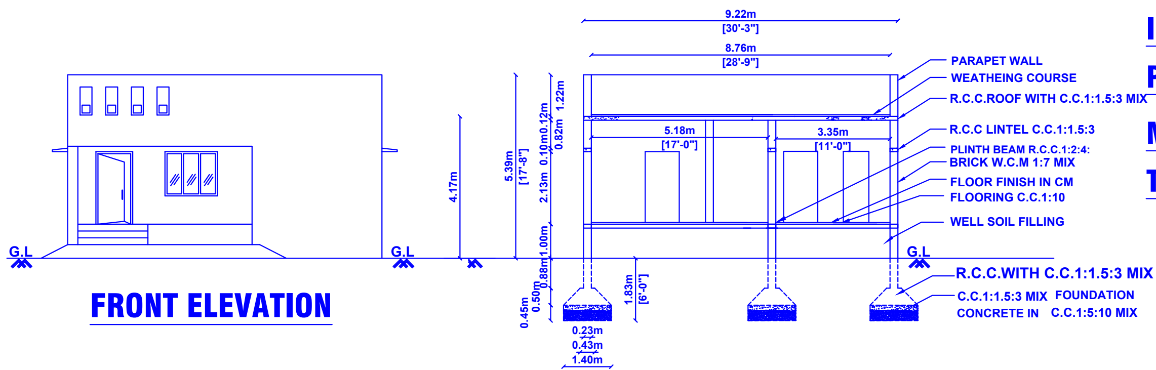
SECTION ON G1G2"
