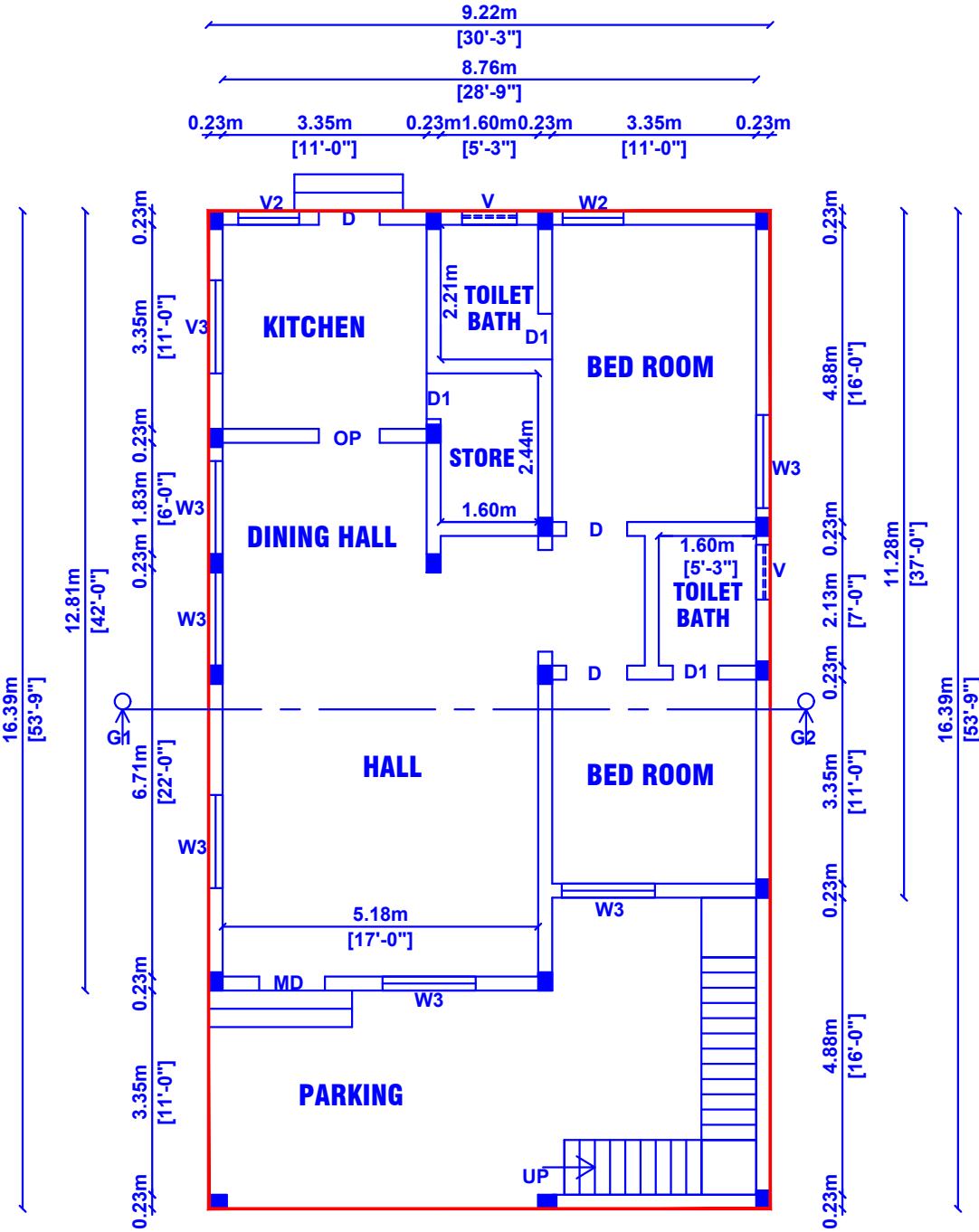
PLAN (Proposed)
