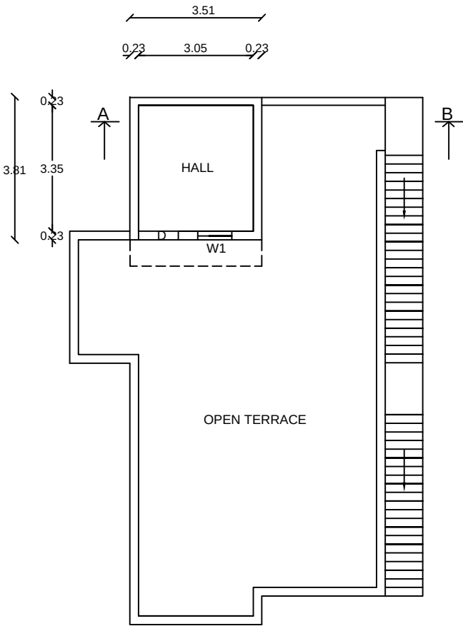
PRO SF PLAN
