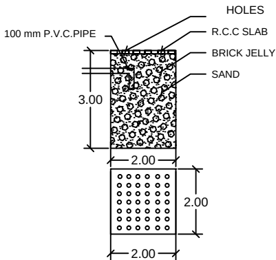
RAIN WATER COLLECTING TANK
