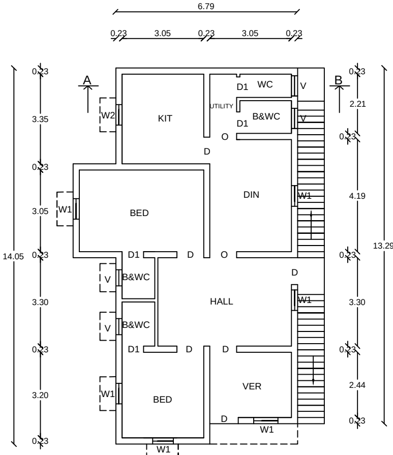
EXG FF PLAN
