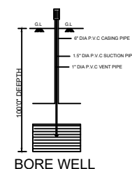
BORE WELL
