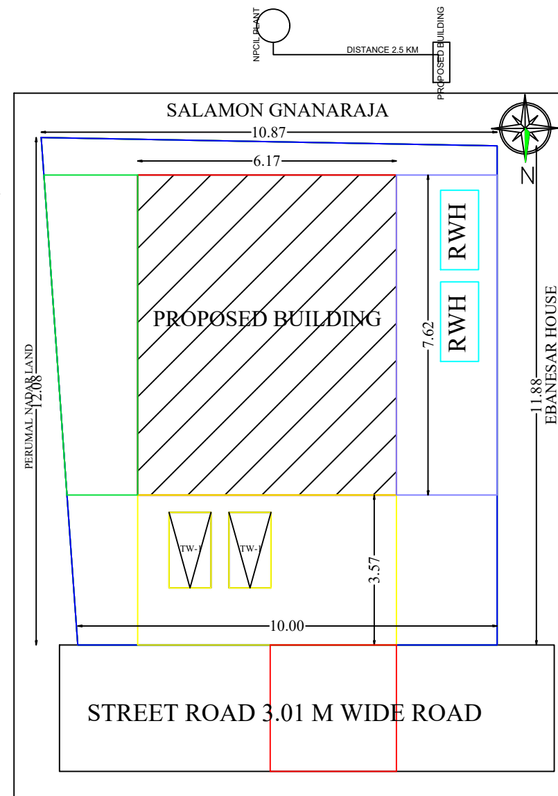
KEY PLAN
