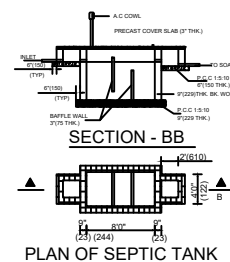
(23) (244) (23) PLAN OF SEPTIC TANK
