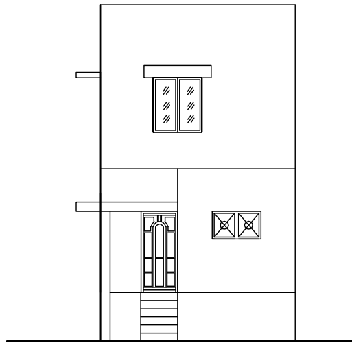
FRONT ELEVATION
