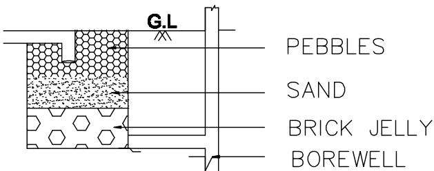
RAINWATER FILTRATION
