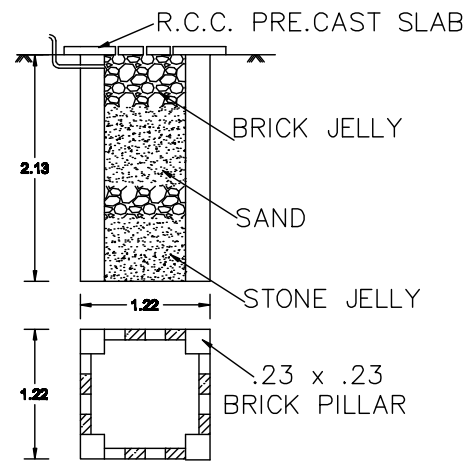
PLAN & SECTION OF RAIN WATER COLLECTION WELL
