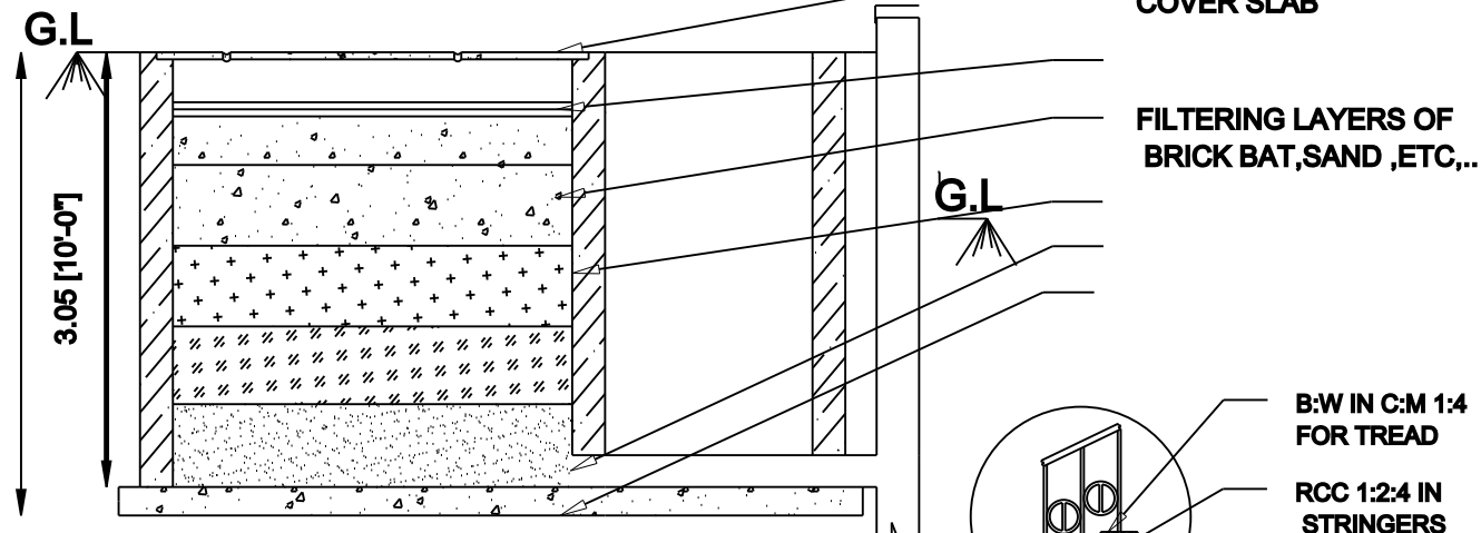
RAIN WATER HARVESTING OF RECHARGE TRENCH METHOD
