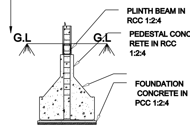
COLUMN DETAILS
