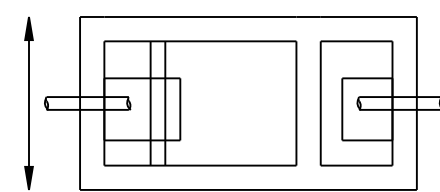
PLAN SEPTIC TANK DETAILS
