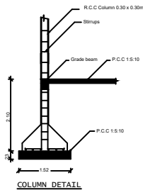
COLUMN DETAIL
