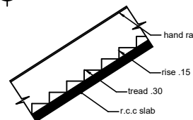
STAIR
