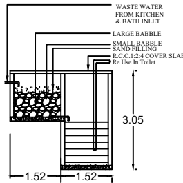
RECYCLING OF WASTE WATER FROM KITCHEN & BATHROOM
