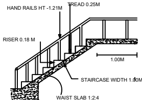
STAIRCASE DETAILS
