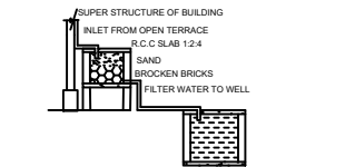
RAINWATER HARVESTING
