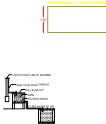
DETAILS OF FILTER BED & WELL NTS
