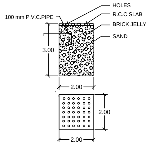
RAIN WATER COLLECTING TANK
