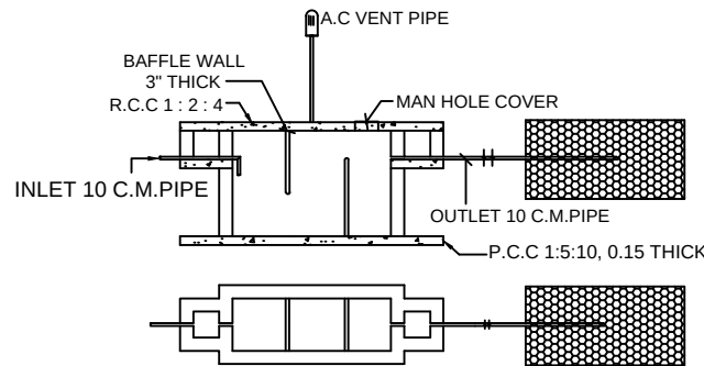
SEPTIC TANK & TRENCH
