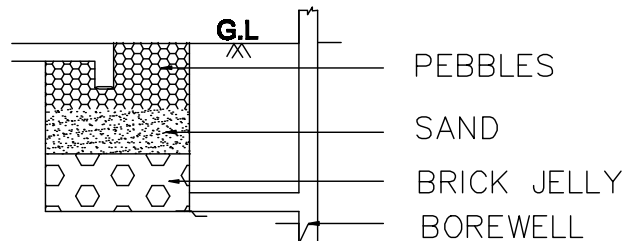
RAINWATER FILTRATION
