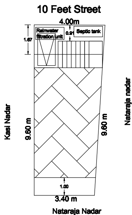
SITE PLAN
