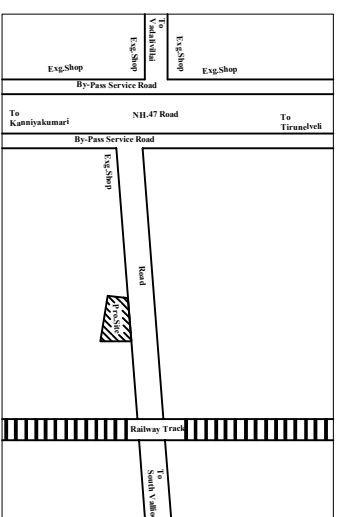
LOCATION PLAN
