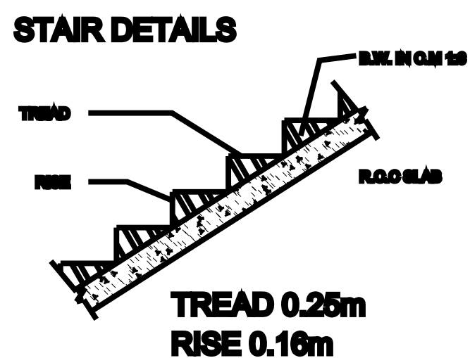
STAIR CASE
