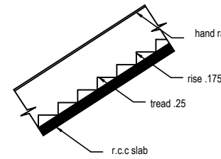
STAIR
