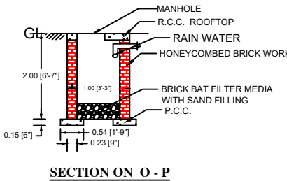
SECTION ON O - P
