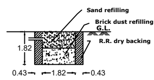
DETAILS OF RAIN WATER HARVESTING Dwg:1A
