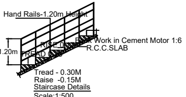
STAIRCASE DETAILS Scale:1:500
