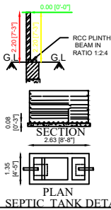
SEPTIC TANK DETAILS
