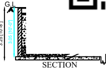
RAIN WATER HARVESTING OF RECHARGE TRENCH METHOD
