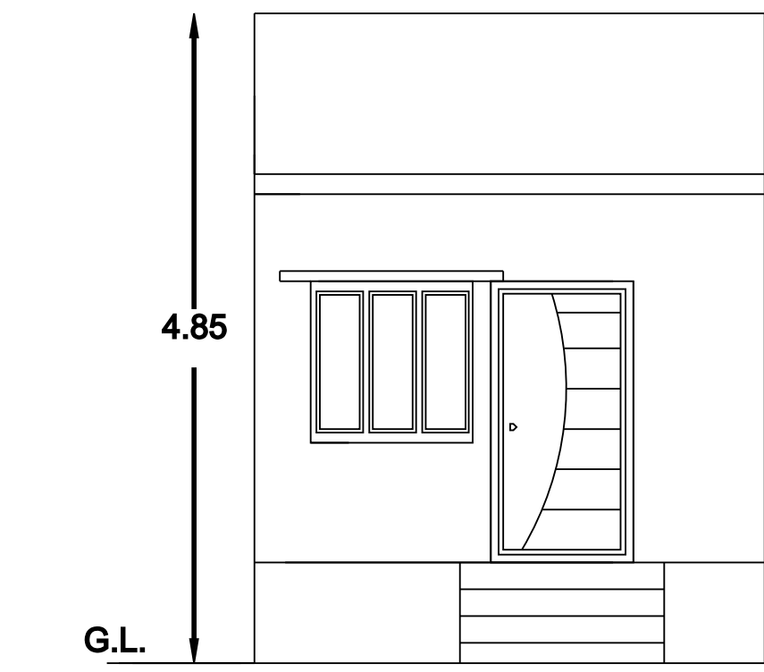
FRONT ELEVATION
